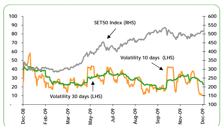
Figure 6: Option Volatility
